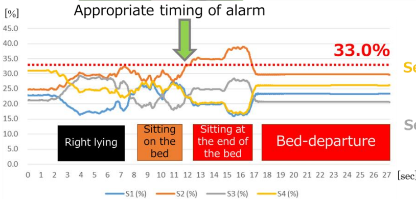
The load ratios applied to each leg of the bed
